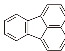
Fluoranthene
