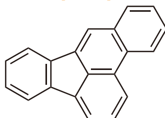
Benzo[b]fluoranthene
